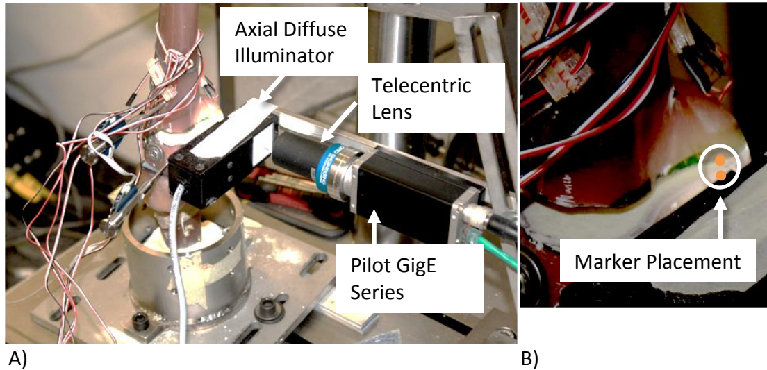
Figure 5.3: Custom tracking system A) A high resolution camera with telecentric lens, and axial diffuse illuminator was used to capture motion of markers placed proximal and distal to the osteotomy (not shown). This system is controlled by a custom LabVIEW program. B) Example of marker placement.
