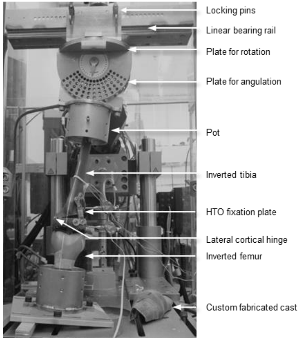
Figure 4.3: Photograph of inverted tibia and femur sawbones mounted in the multi-axis fixation jig. Strain gauges were affixed to the HTO fixation plate and to the lateral cortical hinge.
